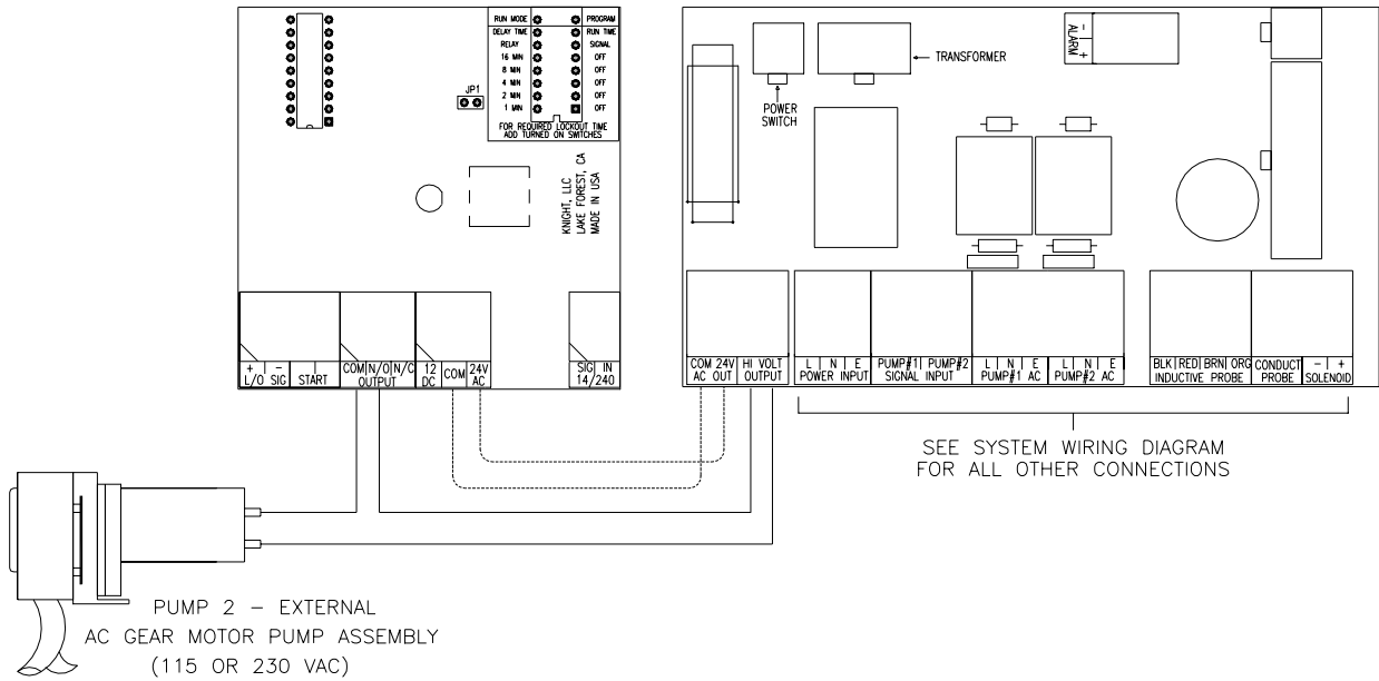
KTM-600 CIRCUIT BOARD
